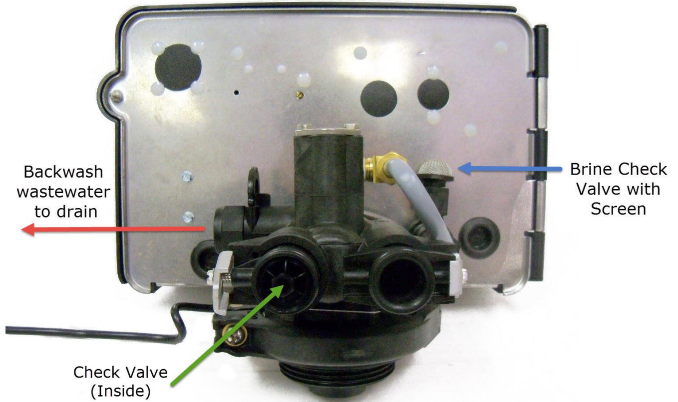
Fig 2 - AIO 2510 SXT Control Valve, Back View
