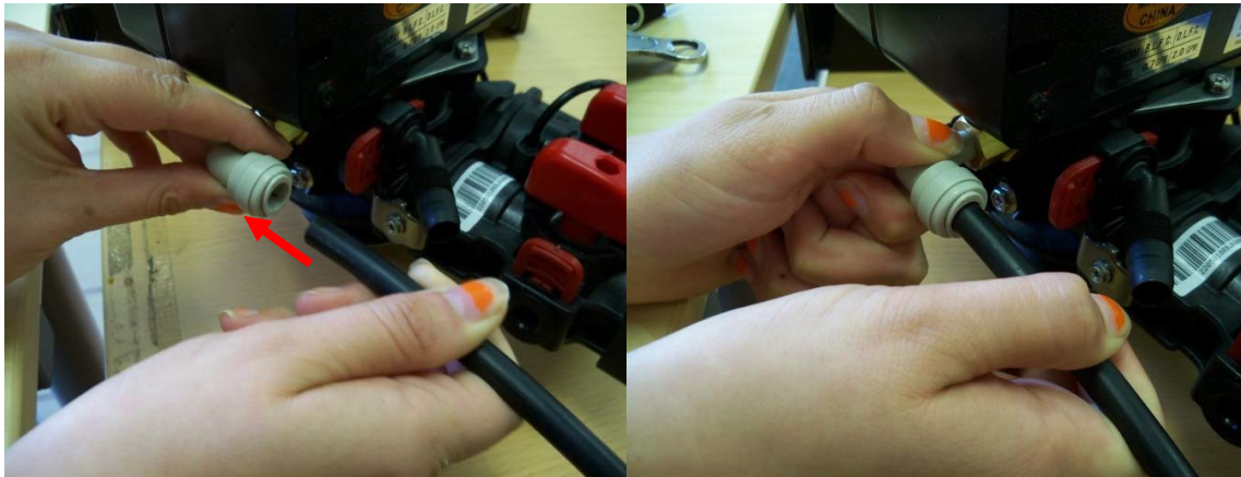
Fig. 6—Pro-OX 1650 Chlorine Side Tank Installation
