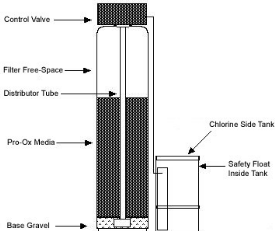
Fig. 1—Iron filter cutaway diagram
