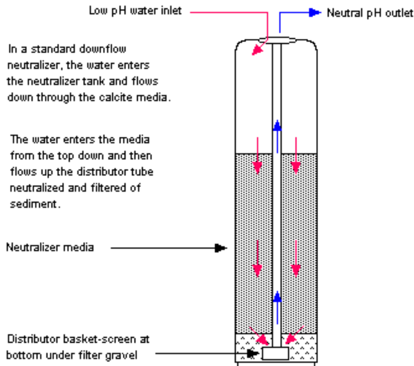
Fig 1 - Calcite Neutralizer Filter Tank Water Flow
