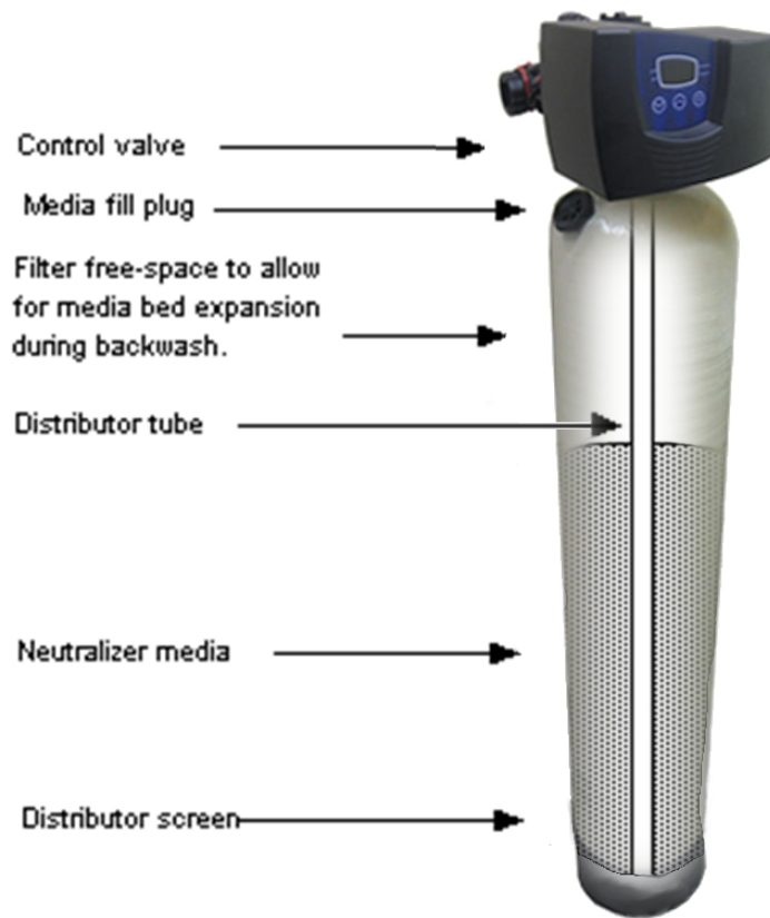
Fig 1 - Calcite Neutralizer Filter Tank Water Flow
