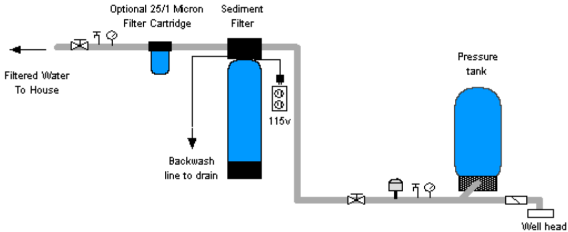
Fig 2: Typical Sediment Filter 5900e piping installation with ball valve and hose bib after the filter
