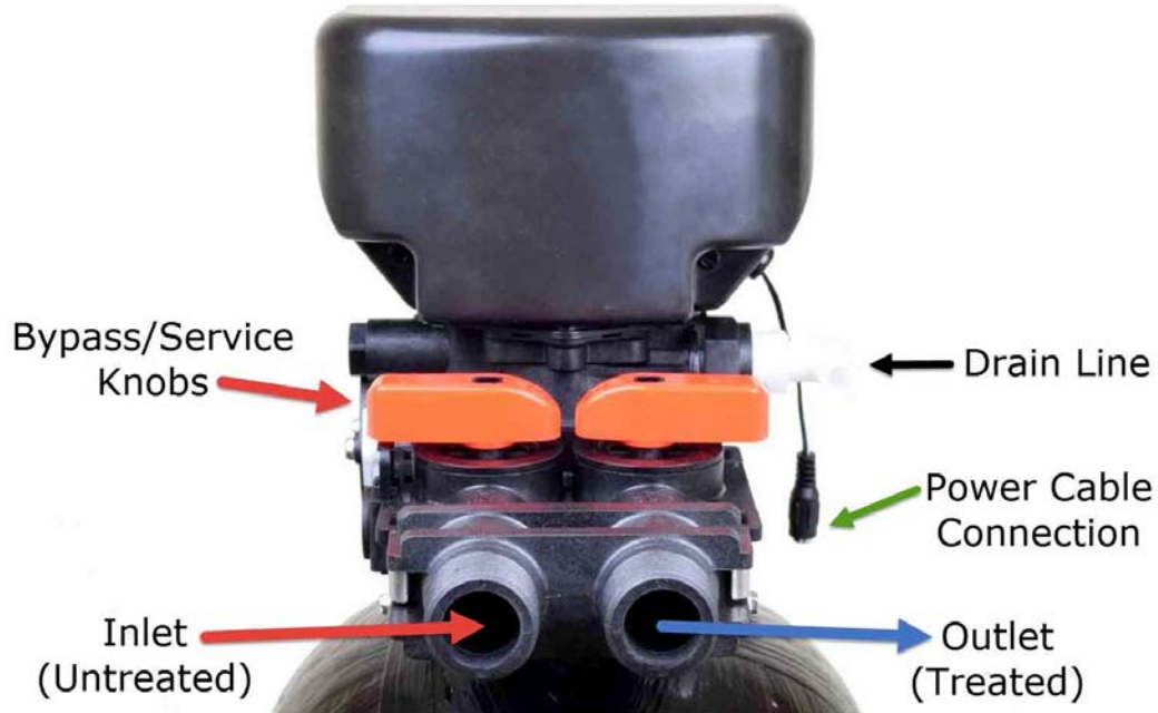
Fig 4: 5900e Bypass/Service Positions
