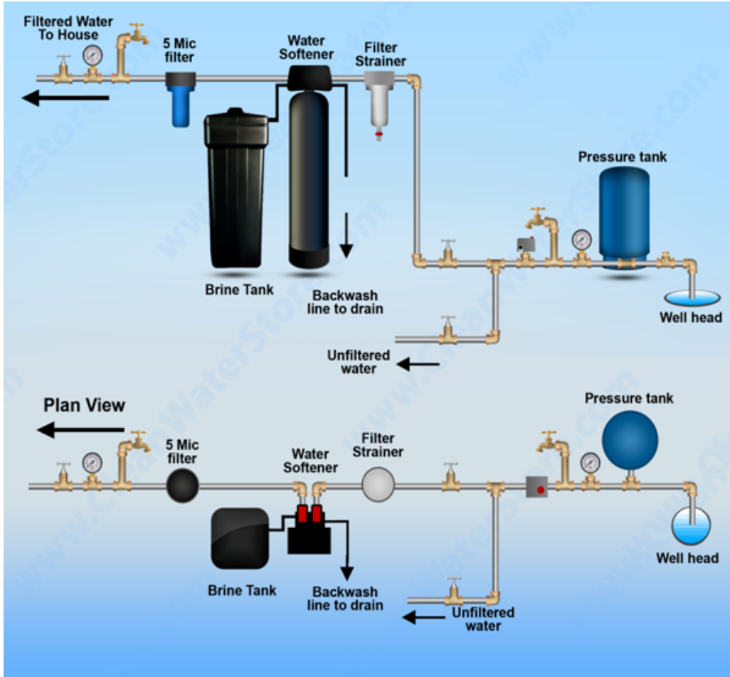
Fig 2 - Typical Softener Fleck 2510 piping installation with ball valve and hose bib after the filter along with pre- and post-filtration if necessary:
