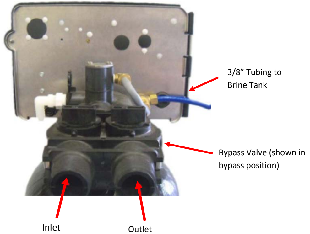
Fig 3: Fleck 2510 from the rear showing the inlet and outlet end-connector fittings 1" or 1-1/4" NPT in Noryl plastic. Brass end-connectors are also available for connecting to copper tubing.
