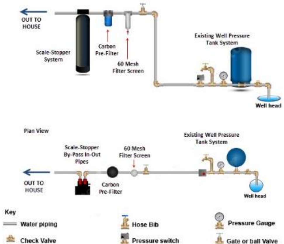
Fig. 2: Recommended Installation for Well Water with the Scale Stopper last in treatment chain, after required carbon filter.
