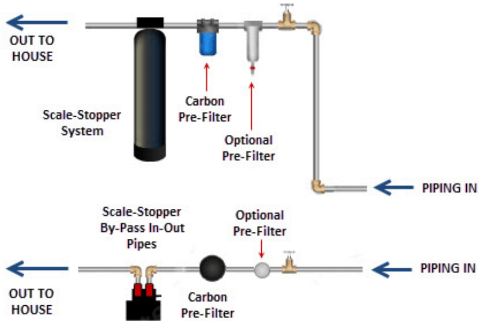
Fig. 1: Recommended Installation for City Water with the Scale Stopper last in treatment chain, after required carbon filter.
