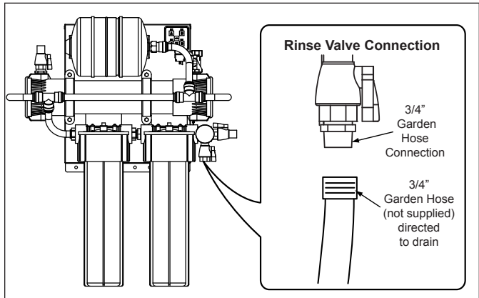
Figure 5. Rinse Valve Connection
