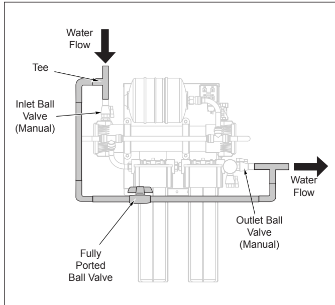
Figure 7. Install Bypass
