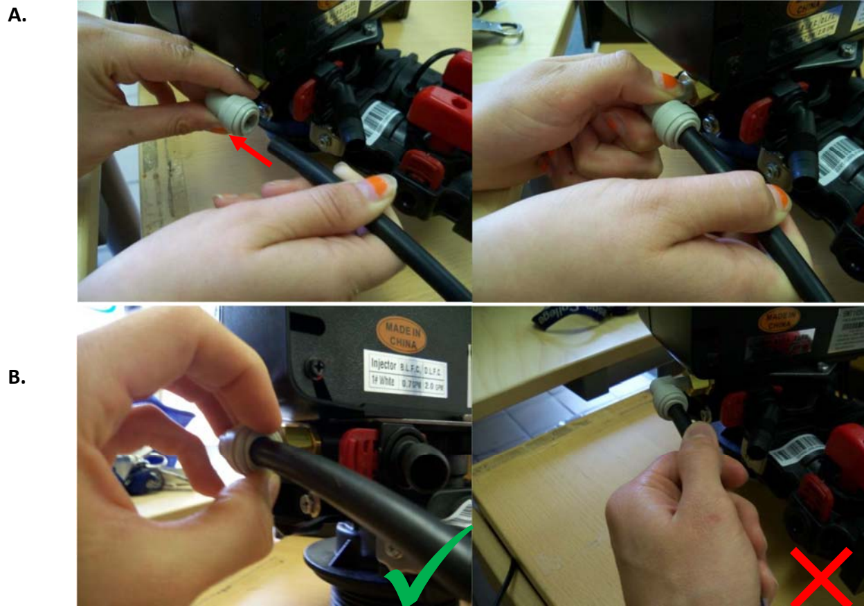
Fig. 6—Pro-OX 1650 Chlorine Side Tank Installation
