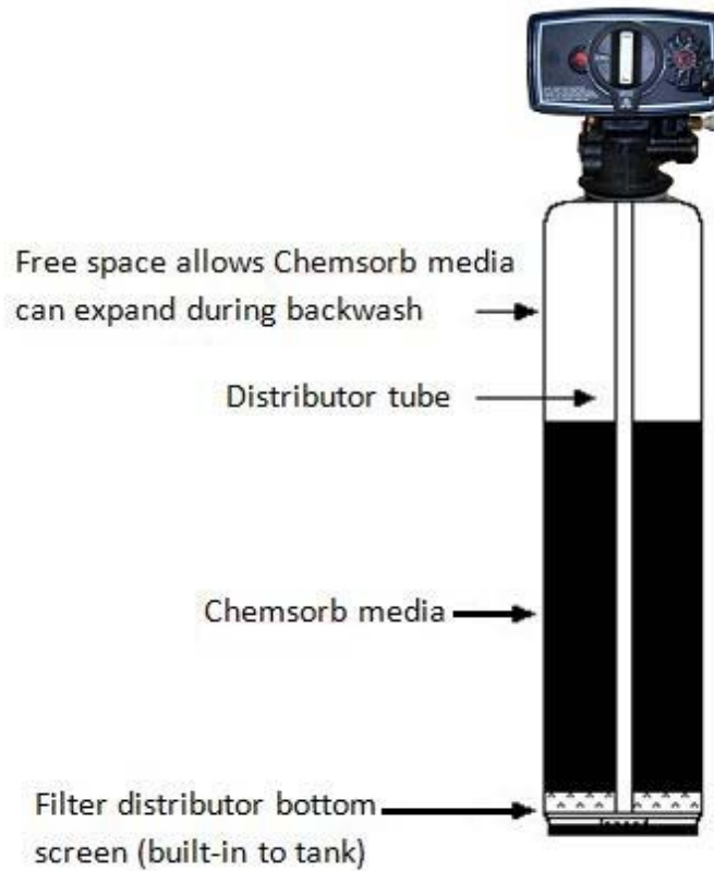
Fig 1: Sediment Filter Tank Water Flow
